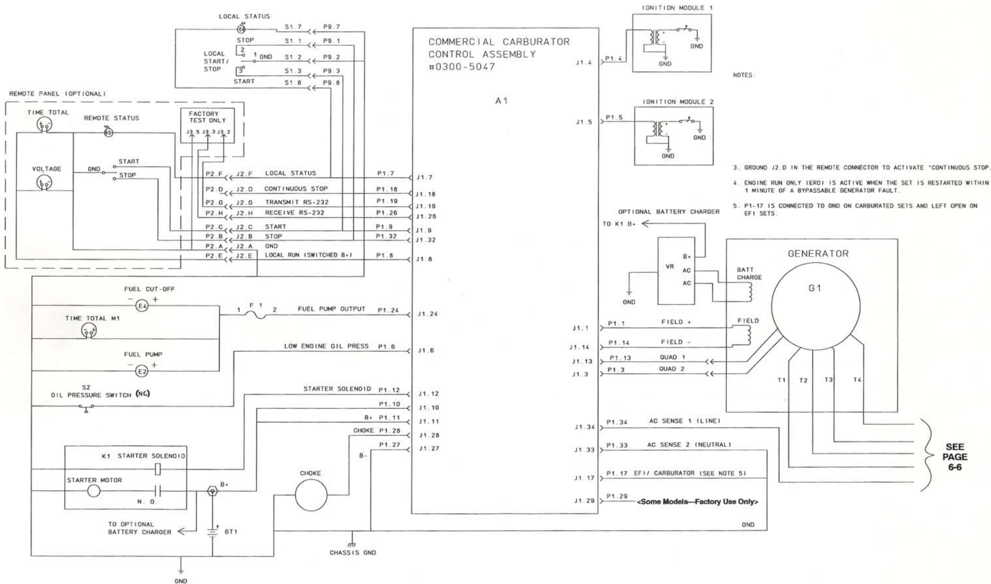
WIRING DIAGRAM—HGJAE & HGJAF
